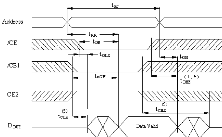
READ CYCLE 3 [1,4]
