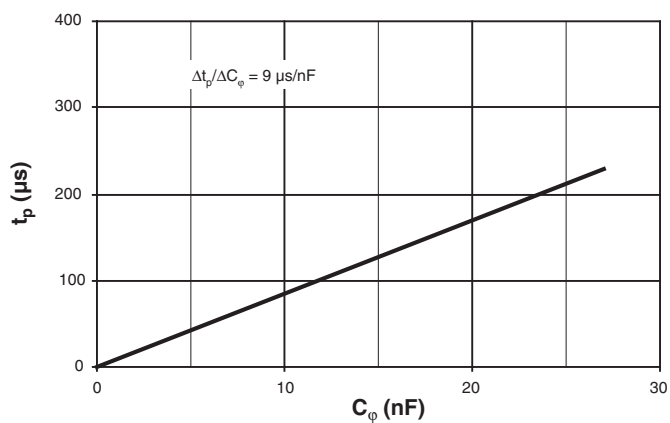
Figure 5-3. Output Pulse Width
