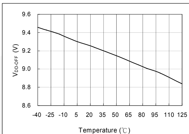
Figure 6. V DD-OFF vs. T A
