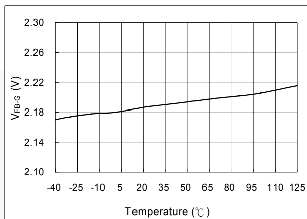
Figure 12. V FB-G vs. T A
