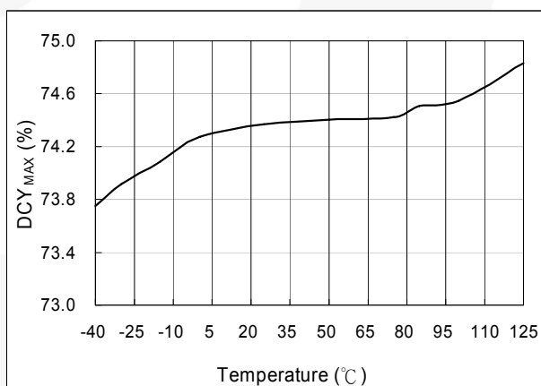
Figure 10. DCY MAX vs. T A
