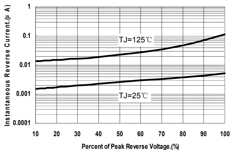
Fig.2-Typical Reverse Characteristics
