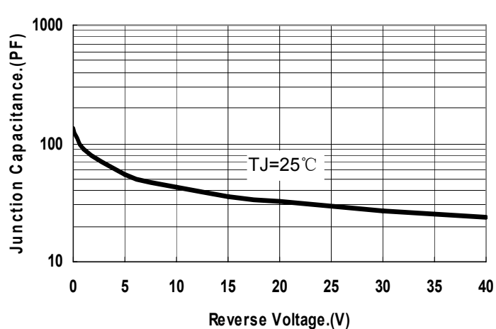
Fig.1-Typical Junction Capacitance
